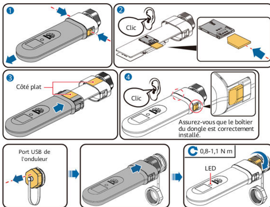
Figure 5-26 Installation du Smart Dongle 4G (SDongleB-06)
