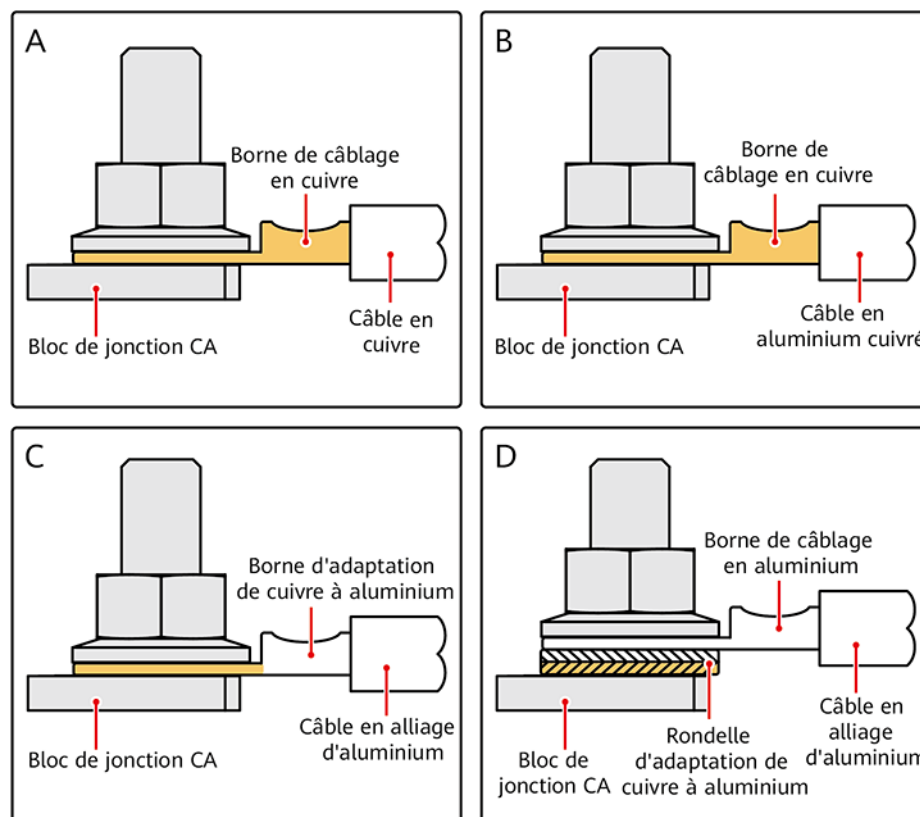
Figure 5-6 Exigences relatives à la borne OT/DT
