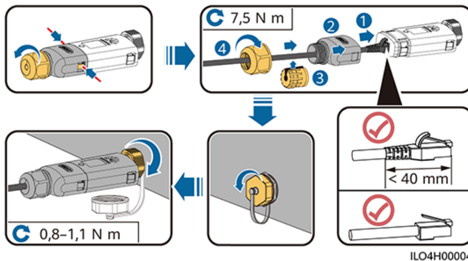
Figure 5-28 Installation du Smart Dongle WLAN-FE (communication FE)
