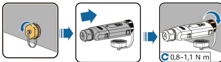
Figure 5-27 Installation du Smart Dongle WLAN-FE (communication WLAN)
