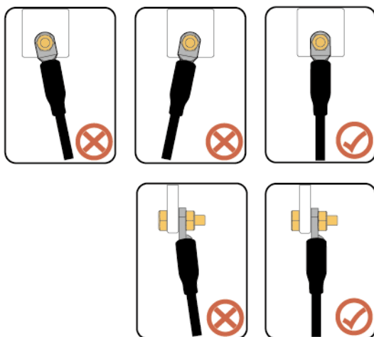
Figure 5-13 Exigences relatives au câblage
