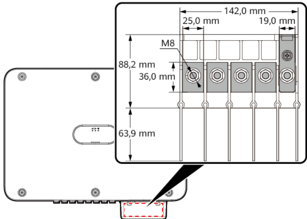
Figure 5-4 Ports de câblage
